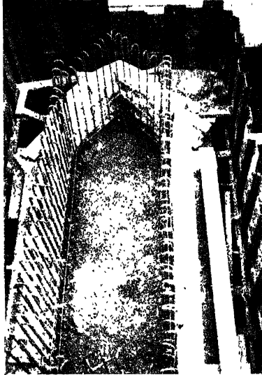
Fig. 154. —Pier Construction within Cofferdam.
